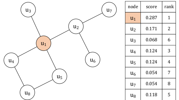
Figure 2: Example of RWR. In the example, the query node is u_1 and RWR scores w.r.t. u_1 are presented in the table. The RWR scores are utilized for personalized ranking or link recommendation for u_1 .
