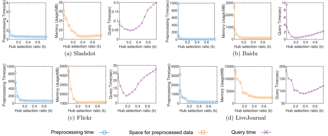
Figure 8: Effects of the hub selection ratio k in Algorithm 3. According to results, preprocessing time and memory usage of BEPI decrease as k increases. Especially, when k is small (e.g., k = 0.001 ), preprocessing time and memory consumption are high. The query speed of BEPI is the fastest when k is around 0.2 \sim 0.3 as shown in the figures.
