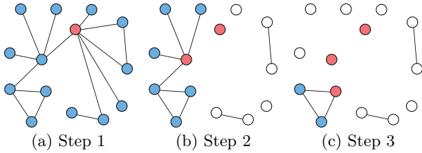
Figure 9: Hub selection in SlashBurn when [kn] = 1 where [kn] indicates the number of selected hubs; red nodes are hubs; white nodes are spokes that belong to the disconnected components; blue colored are nodes that belong to the giant connected component after Step 1.
