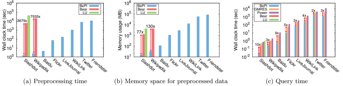
Figure 1: Performance of BEPI: (a) and (b) compare the preprocessing time, and the memory space for preprocessed data, respectively, among preprocessing methods; (c) compares the query time among all tested methods. Bars are omitted if the corresponding experiments run out of memory or time (more than 24 hours). (a) In the preprocessing phase, BEPI is the fastest and the most scalable among all preprocessing methods. Only BEPI successfully preprocesses billion-scale graphs such as Twitter and Friendster datasets. (b) BEPI uses the least amount of space for preprocessed data across all the datasets. Only BEPI preprocesses all the datasets, whereas Bear and LU decomposition fail except for the two smallest ones. (c) In the query phase, BEPI computes RWR scores faster than other competitors over all datasets. Details on these experiments are presented in Section 4.
